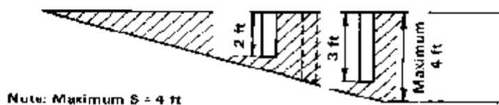
SECTION
