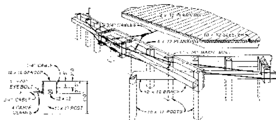
ASSEMBLY PICTORIAL
