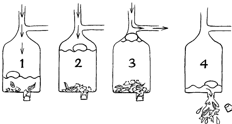
Figure 28: SafeRain system for separating first-flush
