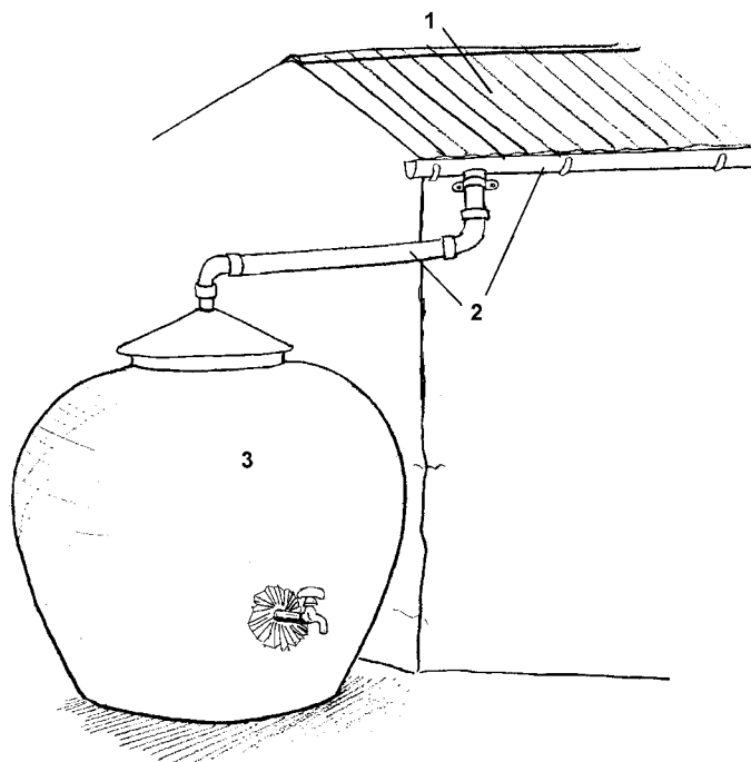
Figure 3: Three basic components of a rainwater harvesting system: catchment (1), delivery system (2), storage reservoir (3)
