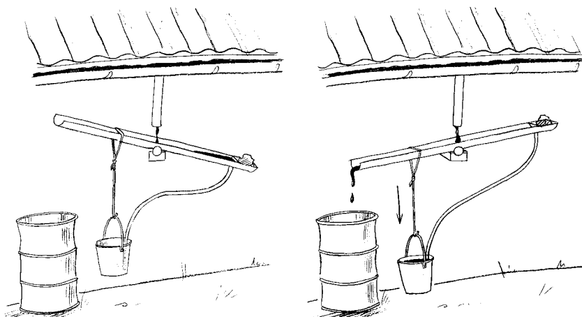
Figure 27: Fixed mass system for separating first-flush relying on the mass of the water
