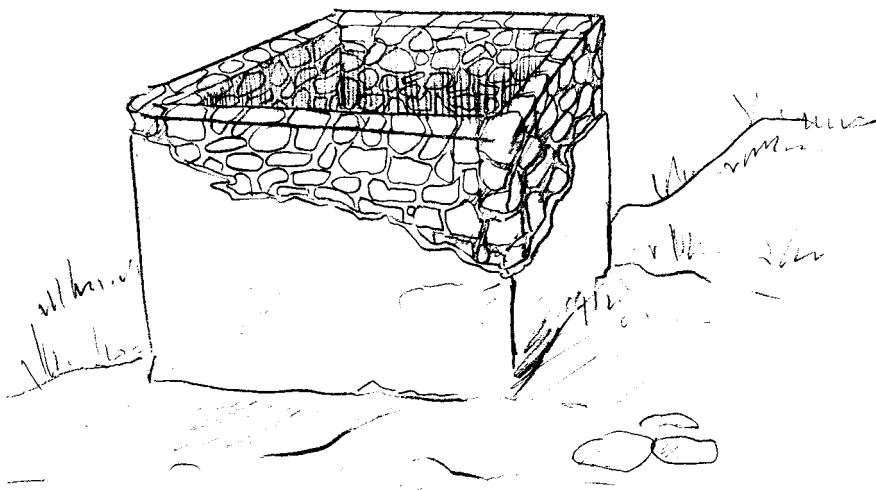
Figure 21: Construction of a water tank built of blocks
