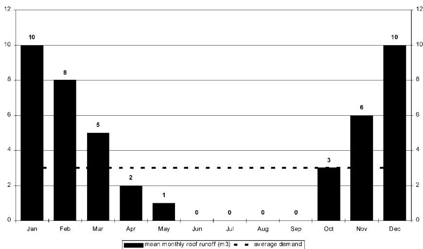
Figure 14: Mean monthly roof run-off and average demand
