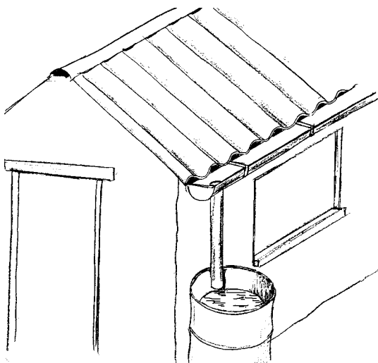
Figure 1: Rainwater harvesting system
