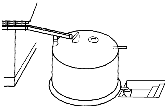
Figure 22: Water tank built of ferro cement with tap at the bottom
