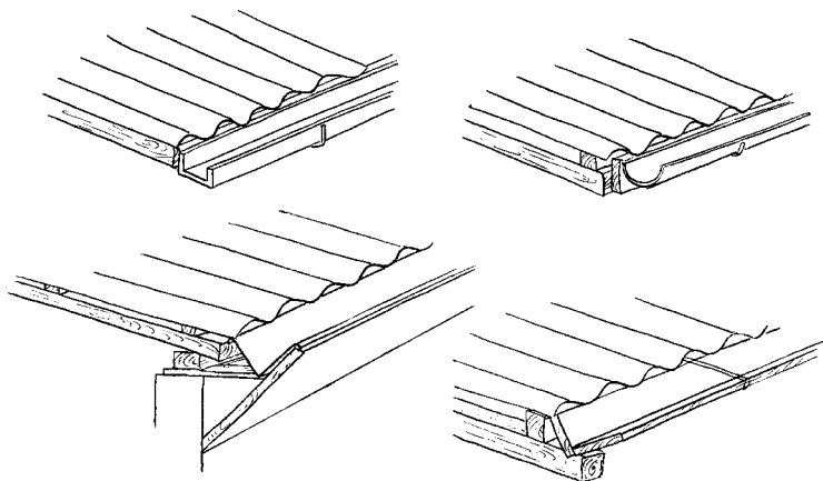
Figure 11: Different types of gutters: square, rounded, V-shaped
