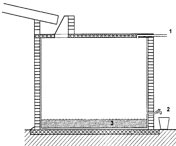
Figure 17: Overflow (1), Tap device (2), Dead storage (3)
