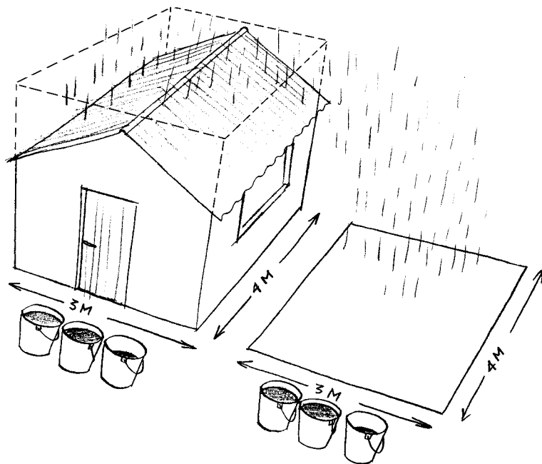
Figure 10: Horizontal plan area of the roof for calculating the catchment surface
