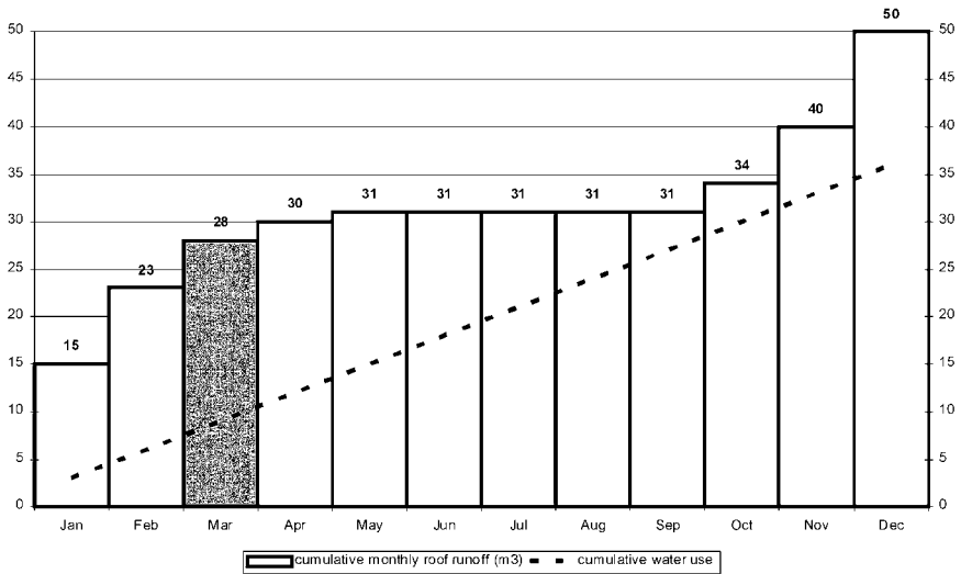
Figure 16: Cumulative monthly roof run-off including a residual storage of 5 m³ and cumulative water use. Estimation of storage requirement.
