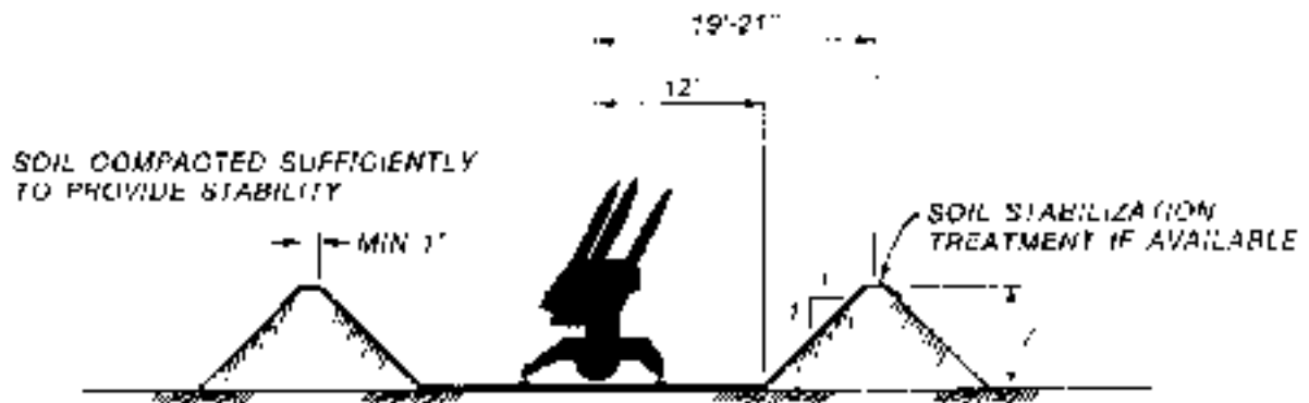
SECTION VIEW
