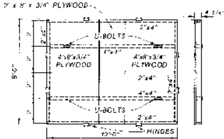
FLOOR DETAIL
