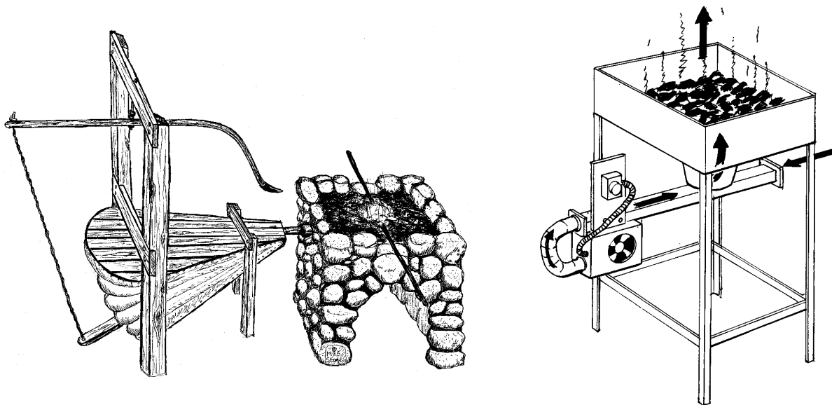
Figure 1. A finished stone forge with an old-time bellows alongside a modern steel backyard forge.
