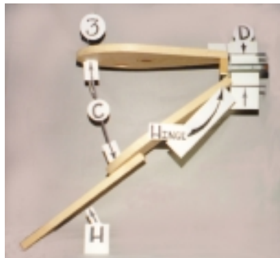
Photograph #3. The bellows handle
