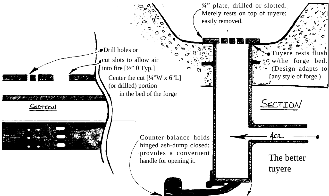
Figure 3. Grate detail
